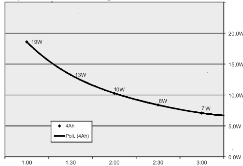
Output Power vs. Discharge Time
